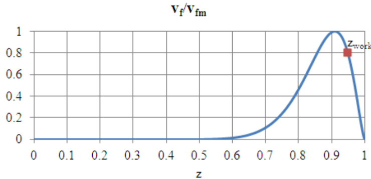
Figure 1. Flame velocity as a function of air molar fraction
