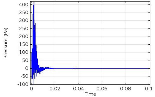
Figure 6. Pressure perturbations. Test case 3
