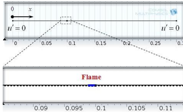
Figure 2. 30-cm configuration
